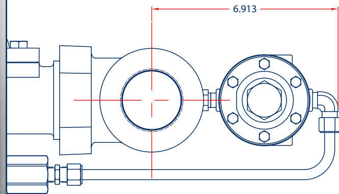
P99 HP Pilot with P39 & Relief Valve
