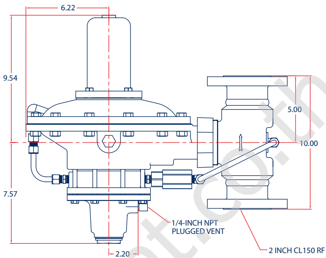
P99 Flanged with Type 61L Pilot
