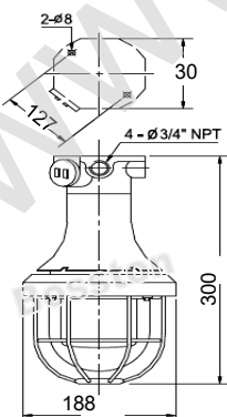
Ceiling mounting
