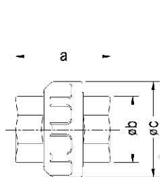
Union 1/2" - 1"
