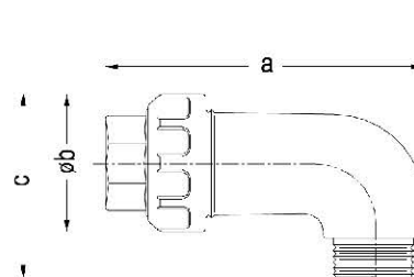
Elbow Union 1/2"-1"
